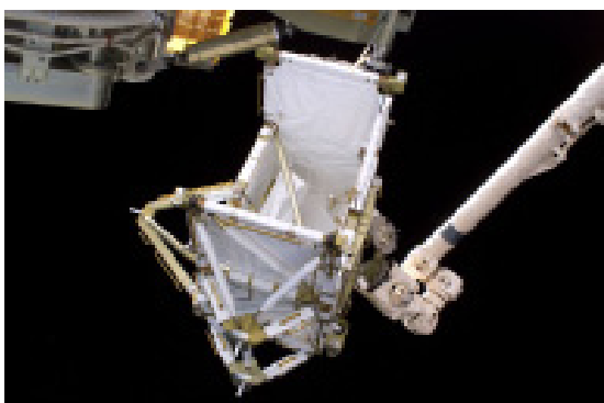
The new P5 truss awaits installation following the hand-off from the shuttle's robotic arm to the station's Canadarm2.
